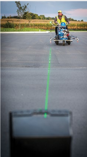
LAZERGUIDE 2000 METHOD: No string line, no chalk and 1 person
